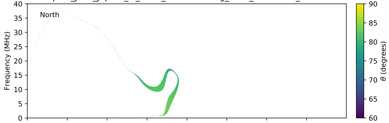
expres_juno_jupiter_io_isaac_lossc-wid1deg_3kev_20160412_v01.cdf
