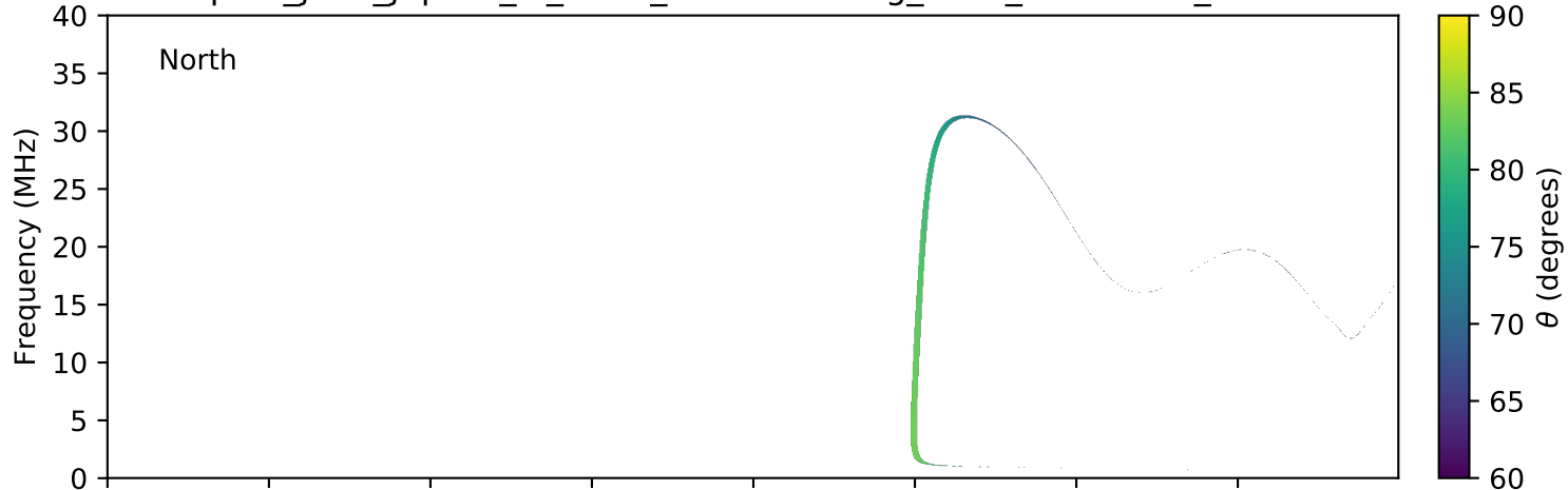
expres_juno_jupiter_io_isaac_lossc-wid1deg_3kev_20160411_v01.cdf
