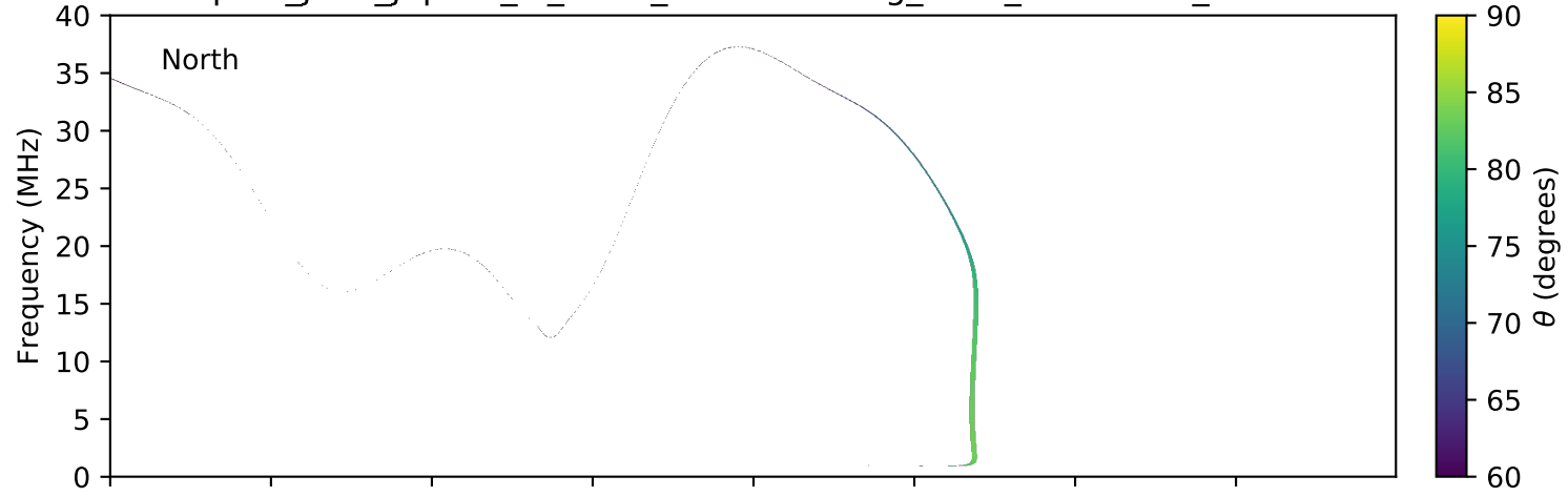
expres_juno_jupiter_io_isaac_lossc-wid1deg_3kev_20160410_v01.cdf
