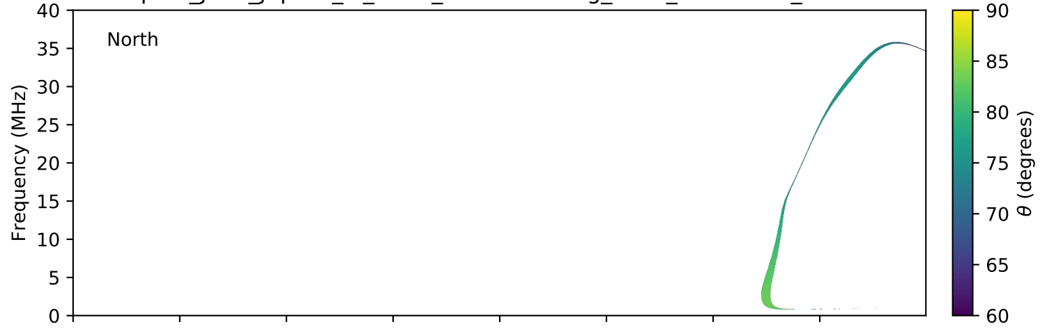
expres_juno_jupiter_io_isaac_lossc-wid1deg_3kev_20160409_v01.cdf
