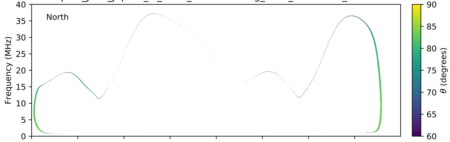
expres_juno_jupiter_io_isaac_lossc-wid1deg_3kev_20160408_v01.cdf
