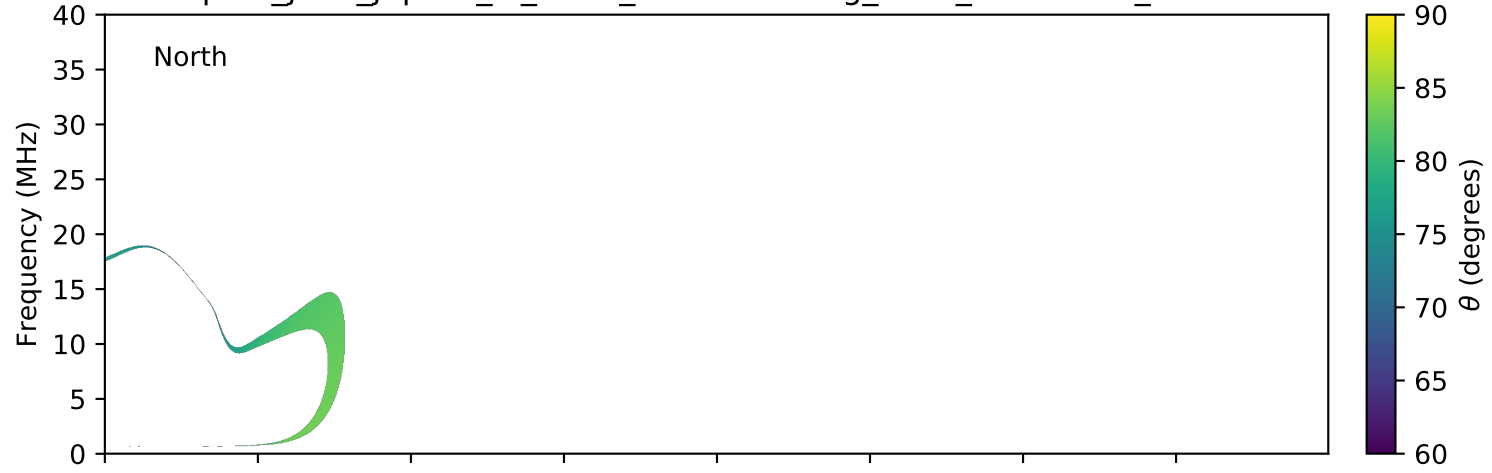
expres_juno_jupiter_io_isaac_lossc-wid1deg_3kev_20160407_v01.cdf
