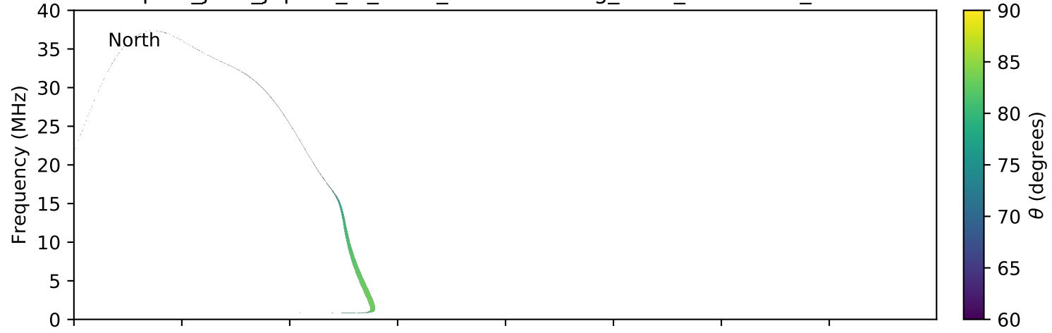
expres_juno_jupiter_io_isaac_lossc-wid1deg_3kev_20160405_v01.cdf
