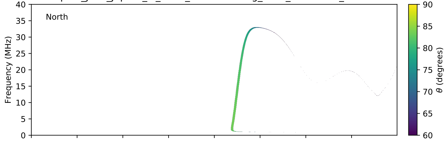
expres_juno_jupiter_io_isaac_lossc-wid1deg_3kev_20160404_v01.cdf
