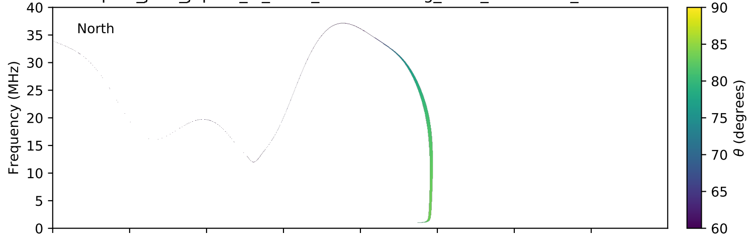
expres_juno_jupiter_io_isaac_lossc-wid1deg_3kev_20160403_v01.cdf
