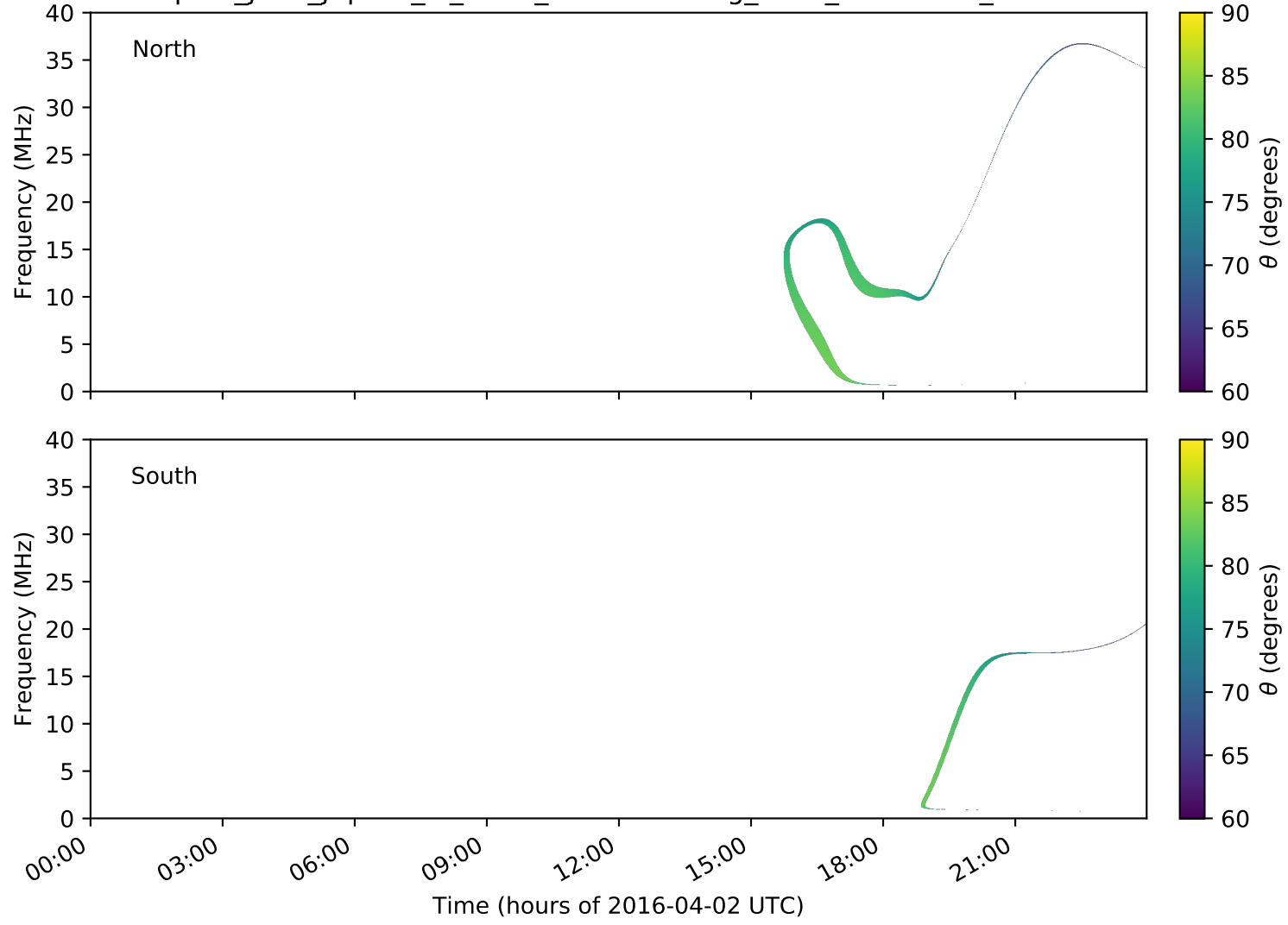
expres_juno_jupiter_io_isaac_lossc-wid1deg_3kev_20160402_v01.cdf
