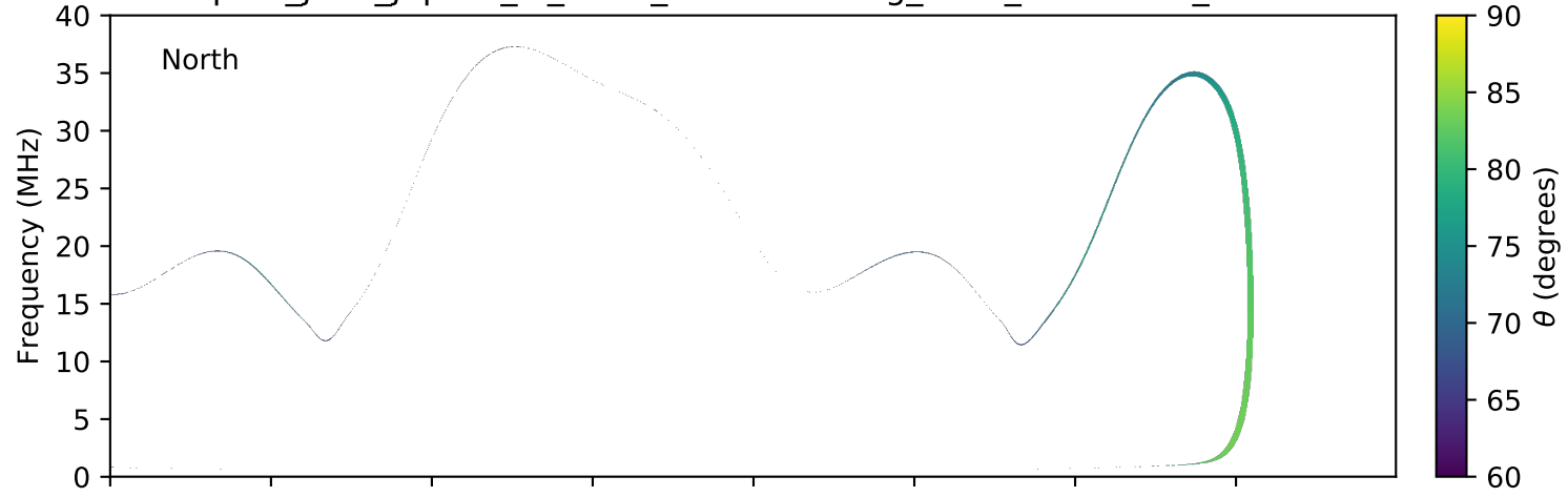
expres_juno_jupiter_io_isaac_lossc-wid1deg_3kev_20160401_v01.cdf
