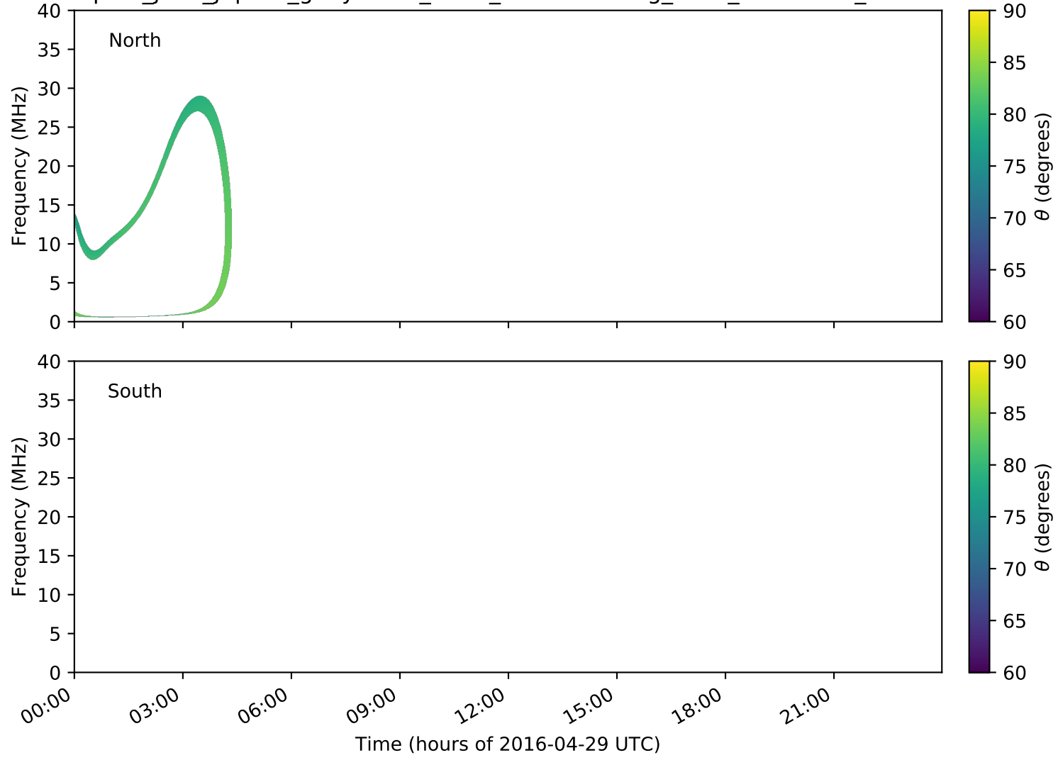
expres_juno_jupiter_ganymede_isaac_lossc-wid1deg_3kev_20160429_v01.cdf
