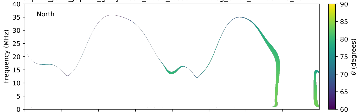
expres_juno_jupiter_ganymede_isaac_lossc-wid1deg_3kev_20160428_v01.cdf
