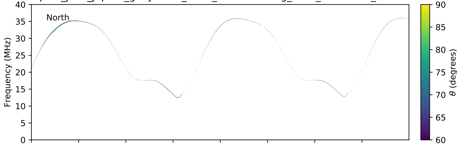
expres_juno_jupiter_ganymede_isaac_lossc-wid1deg_3kev_20160426_v01.cdf
