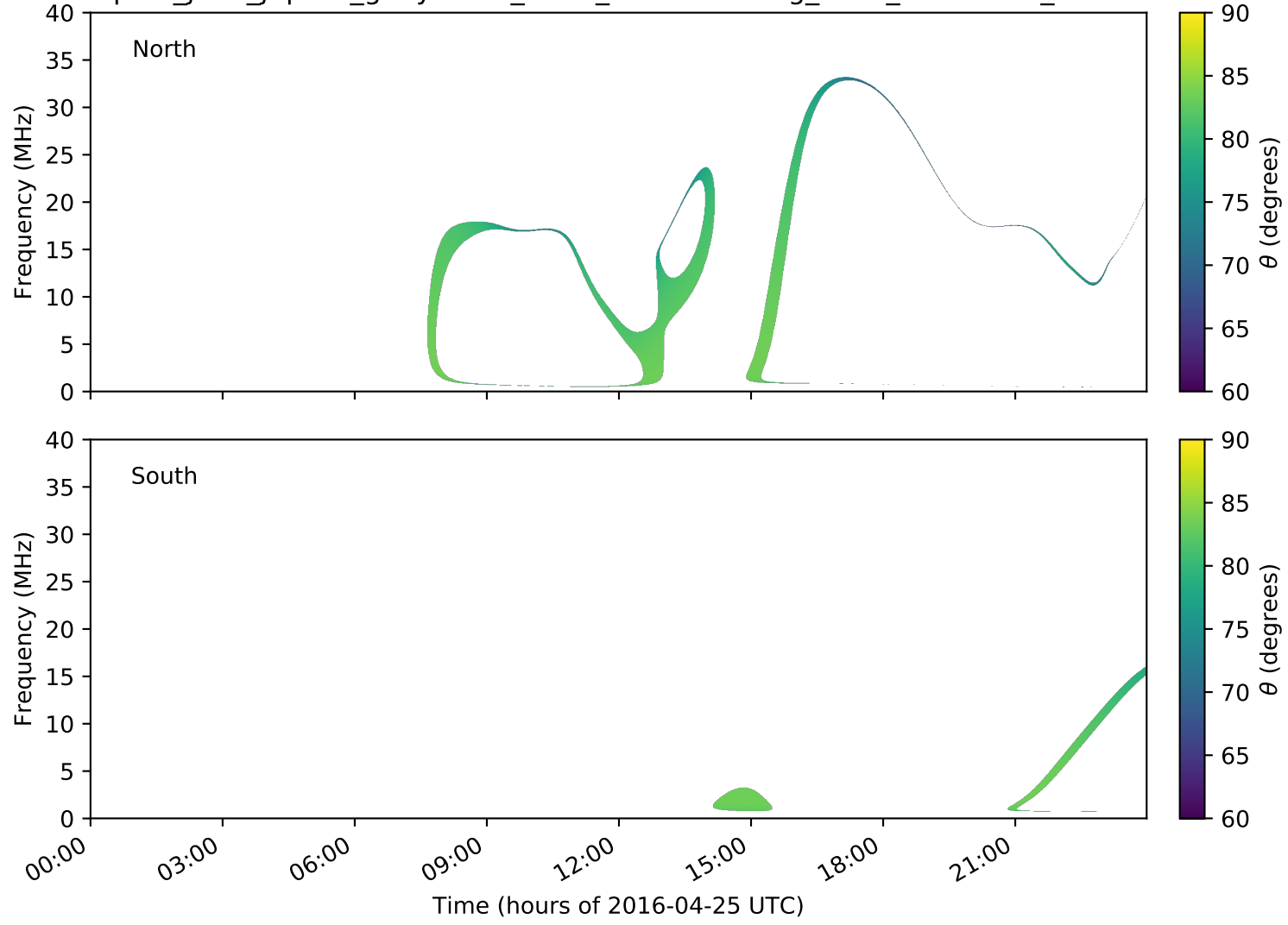
expres_juno_jupiter_ganymede_isaac_lossc-wid1deg_3kev_20160425_v01.cdf
