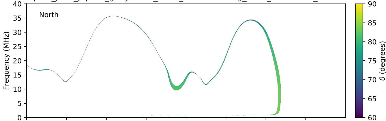
expres_juno_jupiter_ganymede_isaac_lossc-wid1deg_3kev_20160421_v01.cdf
