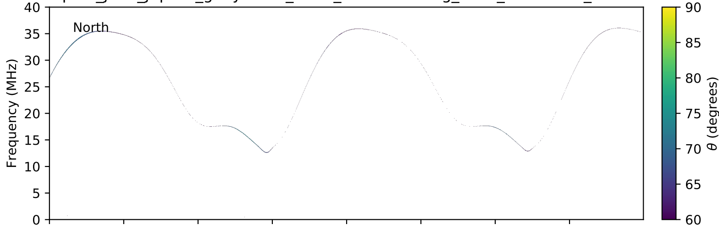
expres_juno_jupiter_ganymede_isaac_lossc-wid1deg_3kev_20160419_v01.cdf
