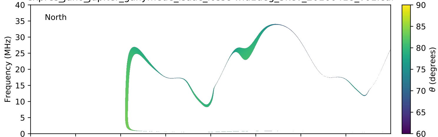
expres_juno_jupiter_ganymede_isaac_lossc-wid1deg_3kev_20160418_v01.cdf
