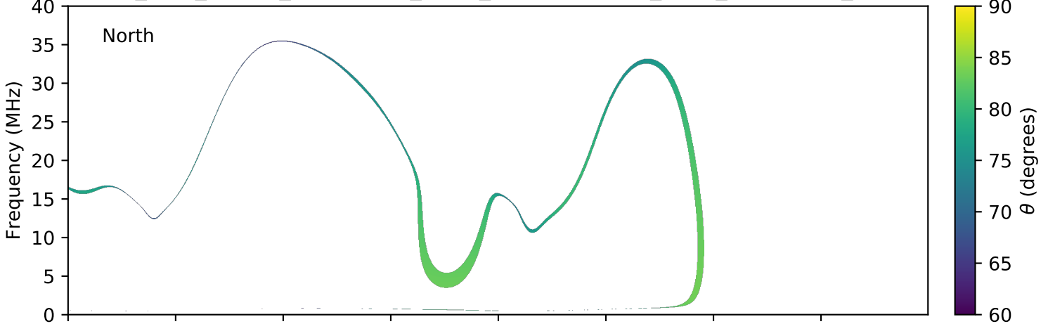
expres_juno_jupiter_ganymede_isaac_lossc-wid1deg_3kev_20160414_v01.cdf
