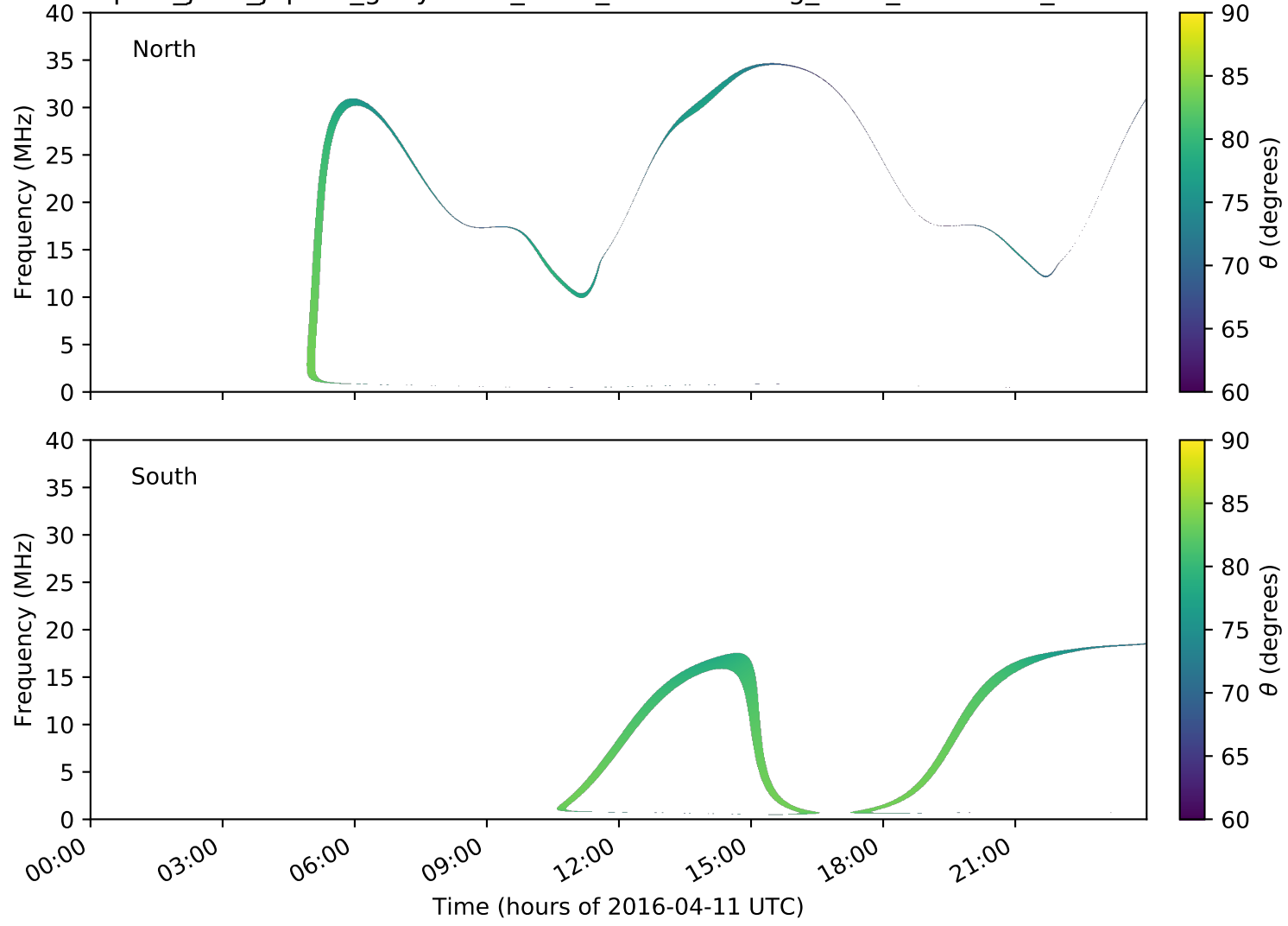
expres_juno_jupiter_ganymede_isaac_lossc-wid1deg_3kev_20160411_v01.cdf
