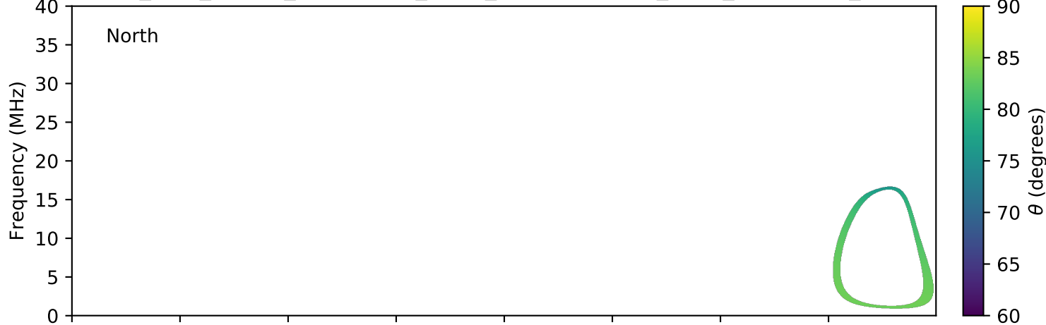
expres_juno_jupiter_ganymede_isaac_lossc-wid1deg_3kev_20160410_v01.cdf
