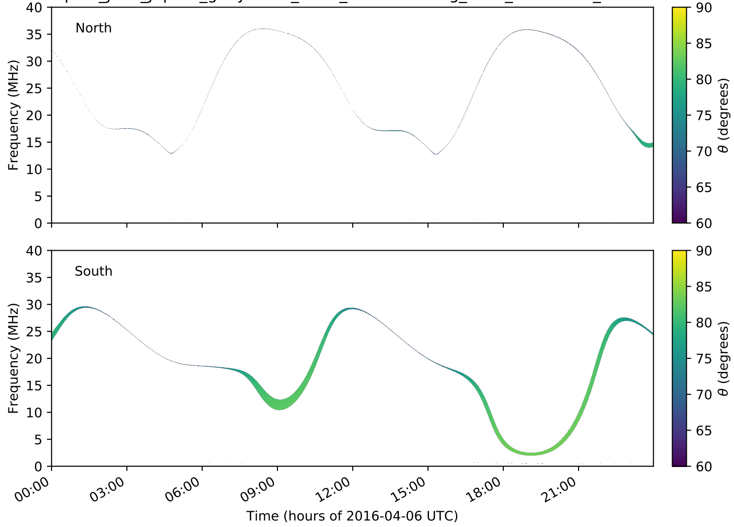
expres_juno_jupiter_ganymede_isaac_lossc-wid1deg_3kev_20160406_v01.cdf
