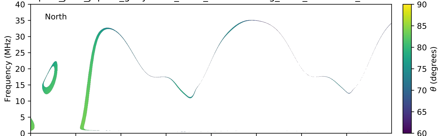
expres_juno_jupiter_ganymede_isaac_lossc-wid1deg_3kev_20160404_v01.cdf
