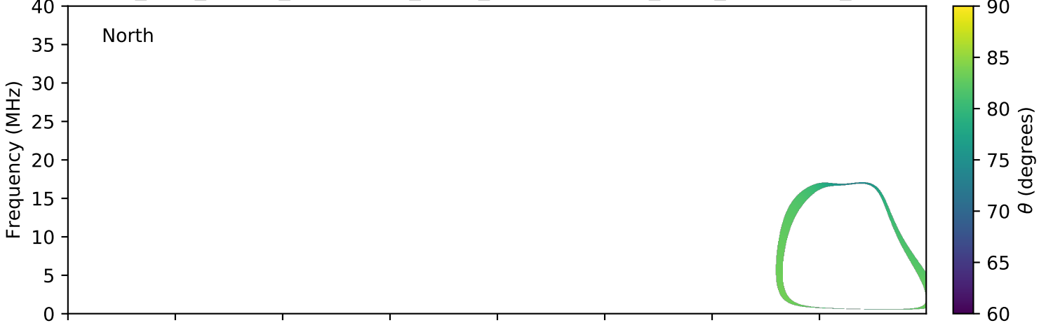
expres_juno_jupiter_ganymede_isaac_lossc-wid1deg_3kev_20160403_v01.cdf
