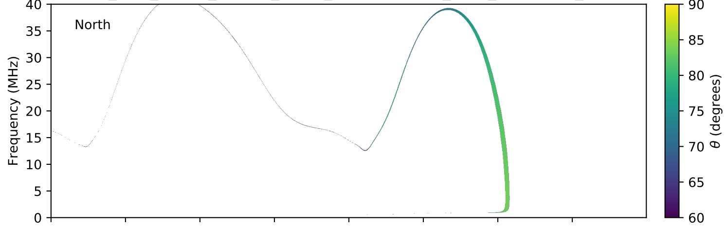
expres_juno_jupiter_europa_jrm09_lossc-wid1deg_3kev_20160426_v01.cdf
