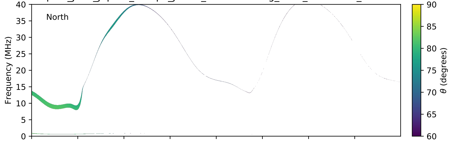
expres_juno_jupiter_europa_jrm09_lossc-wid1deg_3kev_20160425_v01.cdf
