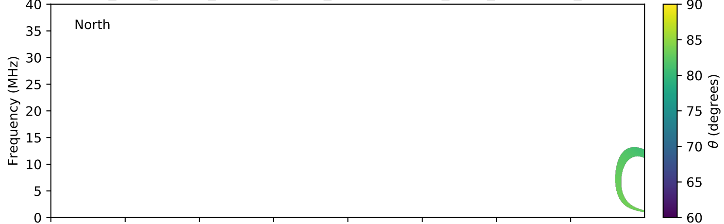
expres_juno_jupiter_europa_jrm09_lossc-wid1deg_3kev_20160424_v01.cdf
