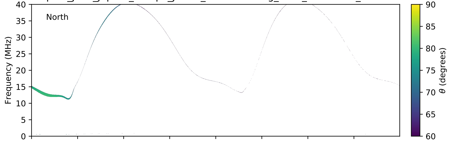
expres_juno_jupiter_europa_jrm09_lossc-wid1deg_3kev_20160418_v01.cdf
