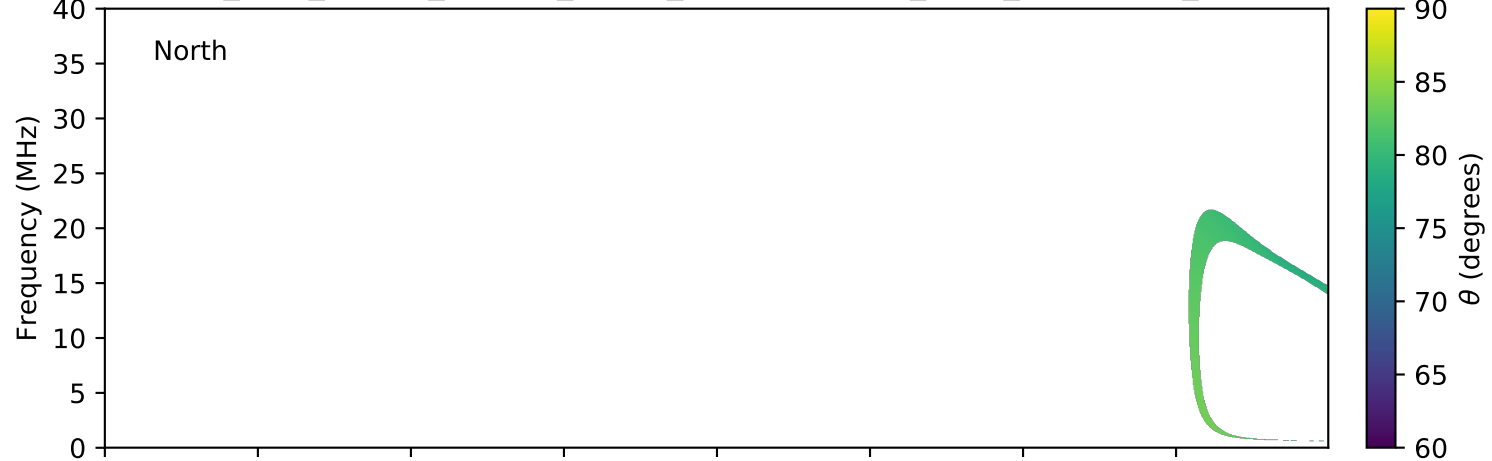
expres_juno_jupiter_europa_jrm09_lossc-wid1deg_3kev_20160417_v01.cdf
