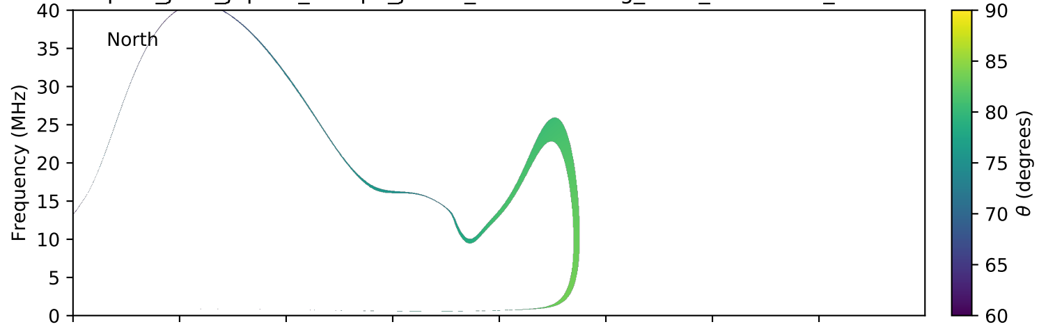
expres_juno_jupiter_europa_jrm09_lossc-wid1deg_3kev_20160405_v01.cdf
