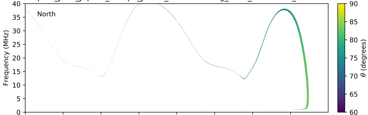
expres_juno_jupiter_europa_jrm09_lossc-wid1deg_3kev_20160401_v01.cdf
