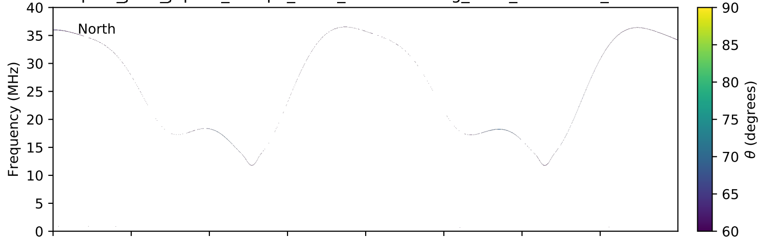
expres_juno_jupiter_europa_isaac_lossc-wid1deg_3kev_20160429_v01.cdf
