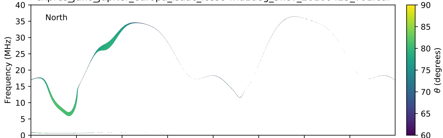
expres_juno_jupiter_europa_isaac_lossc-wid1deg_3kev_20160425_v01.cdf
