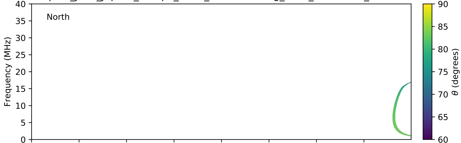
expres_juno_jupiter_europa_isaac_lossc-wid1deg_3kev_20160424_v01.cdf
