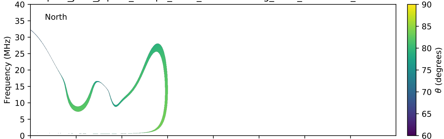
expres_juno_jupiter_europa_isaac_lossc-wid1deg_3kev_20160423_v01.cdf
