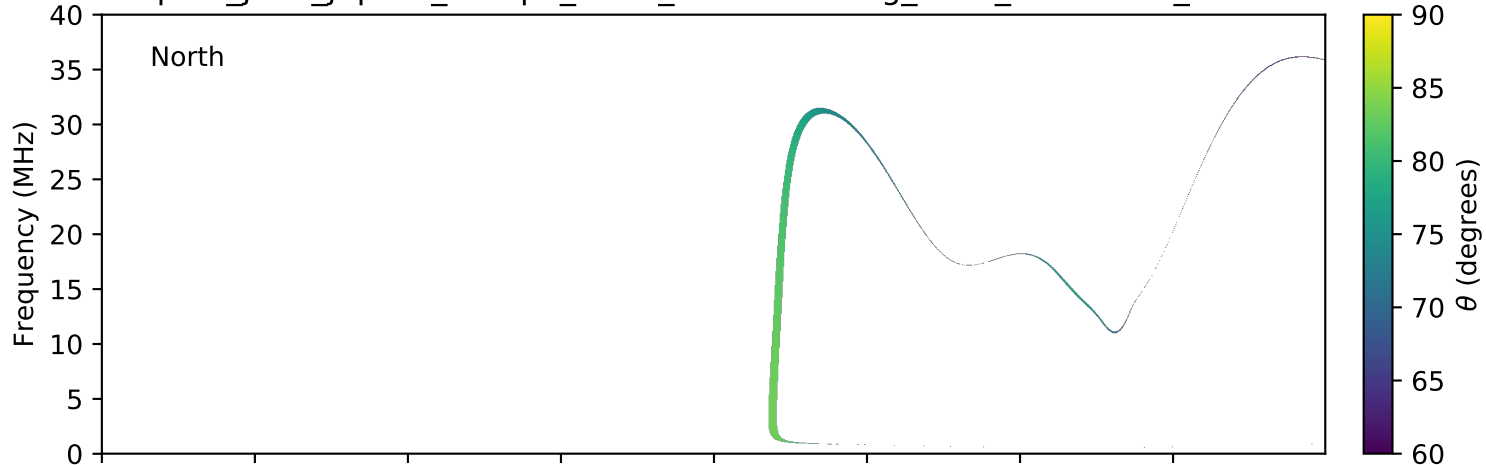
expres_juno_jupiter_europa_isaac_lossc-wid1deg_3kev_20160421_v01.cdf
