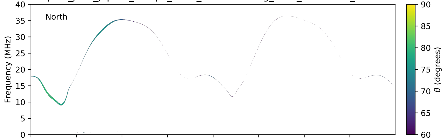
expres_juno_jupiter_europa_isaac_lossc-wid1deg_3kev_20160418_v01.cdf
