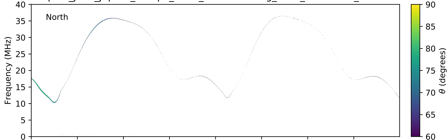
expres_juno_jupiter_europa_isaac_lossc-wid1deg_3kev_20160411_v01.cdf
