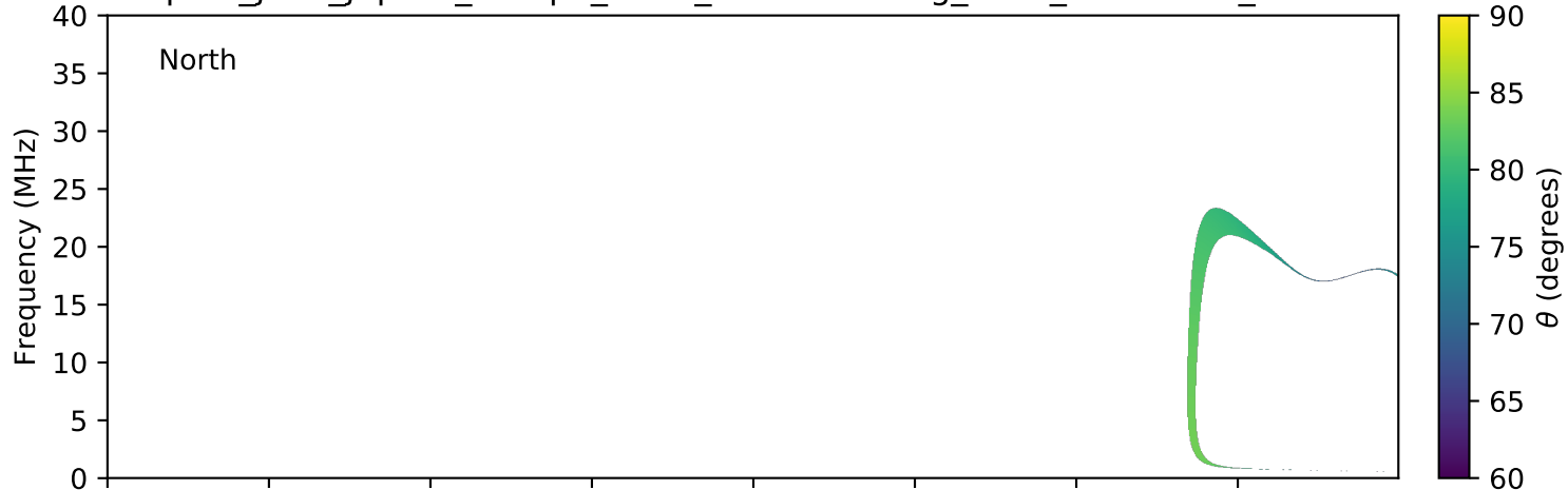
expres_juno_jupiter_europa_isaac_lossc-wid1deg_3kev_20160410_v01.cdf
