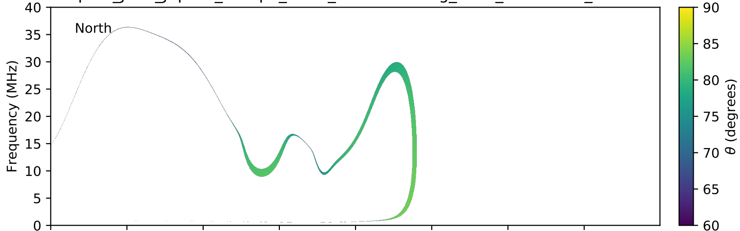
expres_juno_jupiter_europa_isaac_lossc-wid1deg_3kev_20160405_v01.cdf
