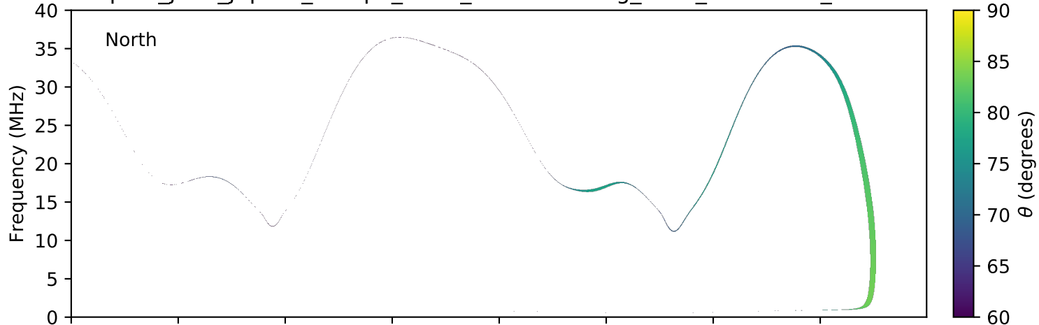
expres_juno_jupiter_europa_isaac_lossc-wid1deg_3kev_20160401_v01.cdf
