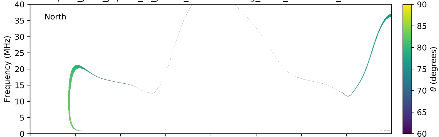
expres_juno_jupiter_io_jrm09_lossc-wid1deg_3kev_20160229_v01.cdf
