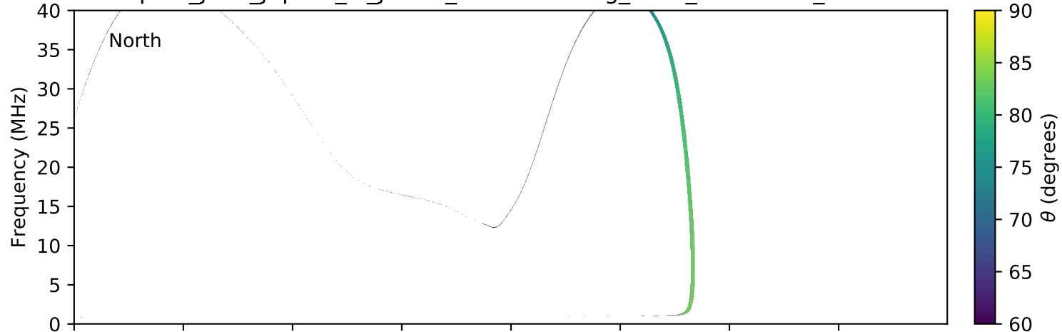
expres_juno_jupiter_io_jrm09_lossc-wid1deg_3kev_20160224_v01.cdf
