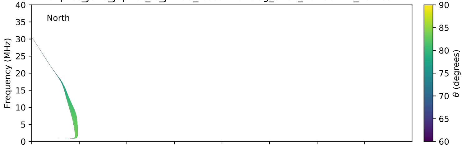
expres_juno_jupiter_io_jrm09_lossc-wid1deg_3kev_20160221_v01.cdf
