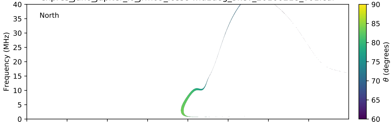
expres_juno_jupiter_io_jrm09_lossc-wid1deg_3kev_20160218_v01.cdf
