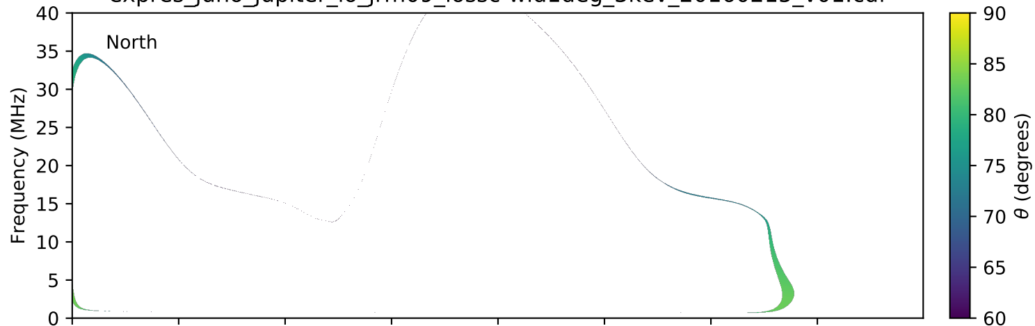
expres_juno_jupiter_io_jrm09_lossc-wid1deg_3kev_20160215_v01.cdf
