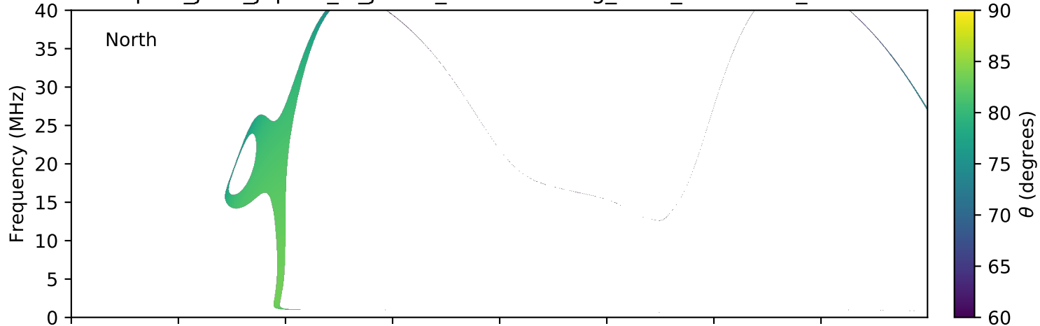
expres_juno_jupiter_io_jrm09_lossc-wid1deg_3kev_20160213_v01.cdf
