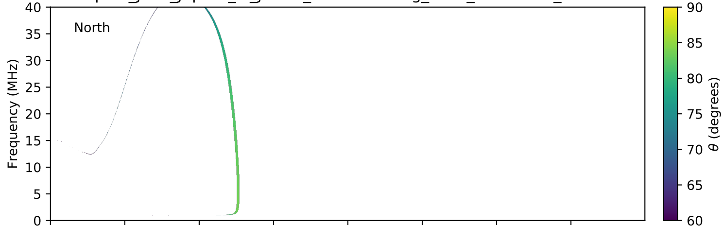
expres_juno_jupiter_io_jrm09_lossc-wid1deg_3kev_20160212_v01.cdf
