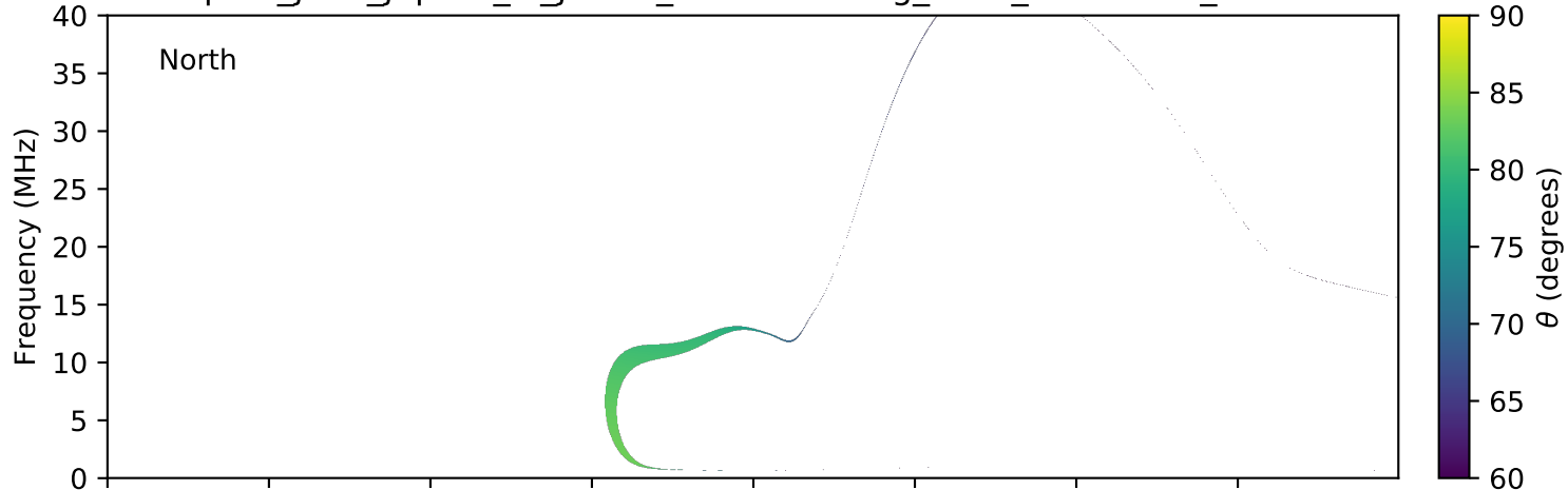
expres_juno_jupiter_io_jrm09_lossc-wid1deg_3kev_20160211_v01.cdf
