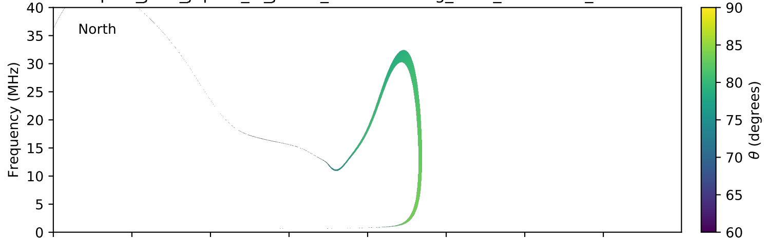
expres_juno_jupiter_io_jrm09_lossc-wid1deg_3kev_20160210_v01.cdf
